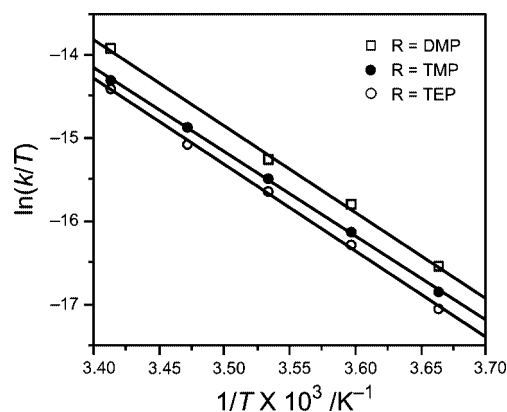
Figure 4. Eyring plots for the stereomutation of O - cis 2k–m to O - trans 3k–m in toluene at 273–293 K.
