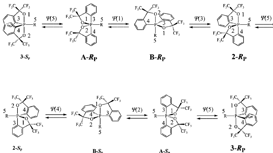
Figure 2. A multi-step pseudorotation process between the most stable isomers, O-trans 3-S P and 3-R P
