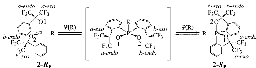
Figure 1. Interconversion between enantiomers 2-R P and 2-S P by a single step pseudorotation. The groups designated exo and endo cannot interconvert with this process.
