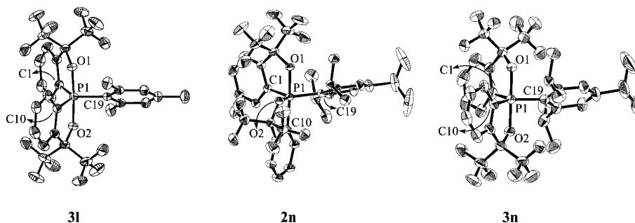
Figure 3. The ORTEP drawings of 3l (left), 2n (middle), and 3n (right) showing the thermal ellipsoids at the 30% probability level. All the hydrogens have been omitted for clarity.
