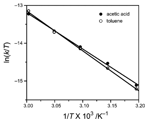
Figure 5. Eyring plot for the stereomutation of O - cis 2n to O - trans 3n in toluene and in acetic acid at 313–333 K.
